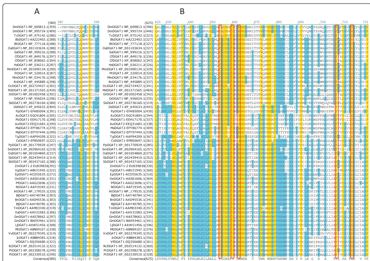
Figure 4 Identification of completely conserved amino acid residues in sequence motifs 4-5 of DGAT1s. (A) DGAT1-Motif 4 (QP Block), (B) DGAT1-Motif 5 (LWLFEEFDFRYWWNNWNPFSHP Block); The first boxed F residues are also conserved in DGAT2s; The boxed Y, W and the second F residues are mutated in TmDGAT1 and the boxed H residue is mutated in MmDGAT1). Refer to Figure 3 legend for additional information.
